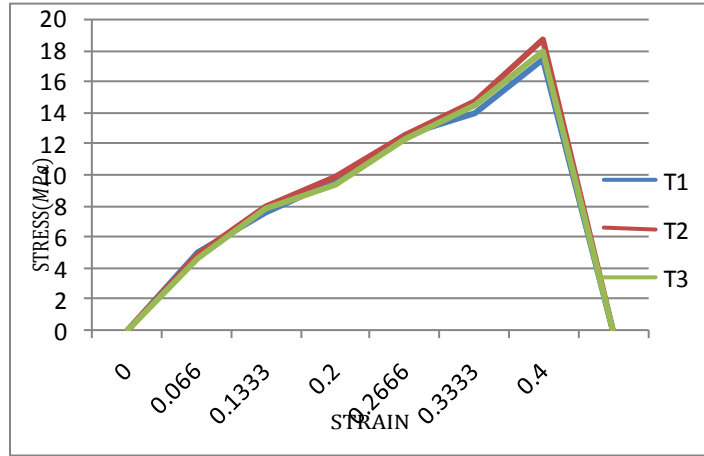
Fig.7 Stress vs Strain graph of Tensile test for composition 65%-35%
