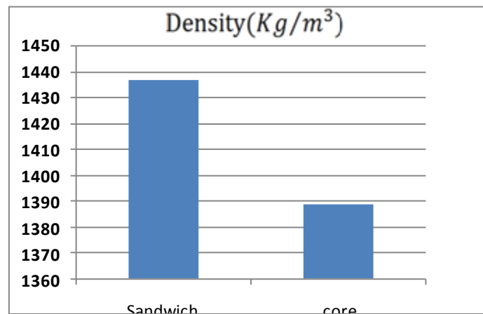
Figure 5: Comparison result of core and sandwich composite results
