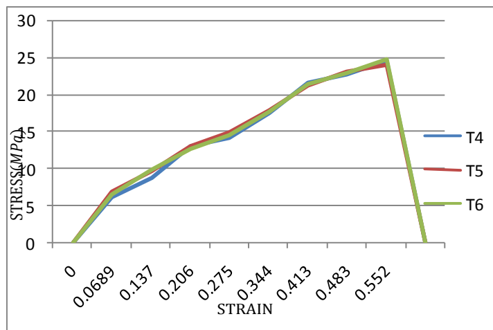
Fig 9. Stress vs Strain graph Tensile test for composition 60%-40%
