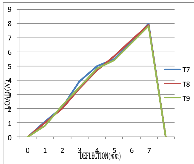
Fig 10 Load vs Deflection graph of Tensile test for composition 55%-45%
