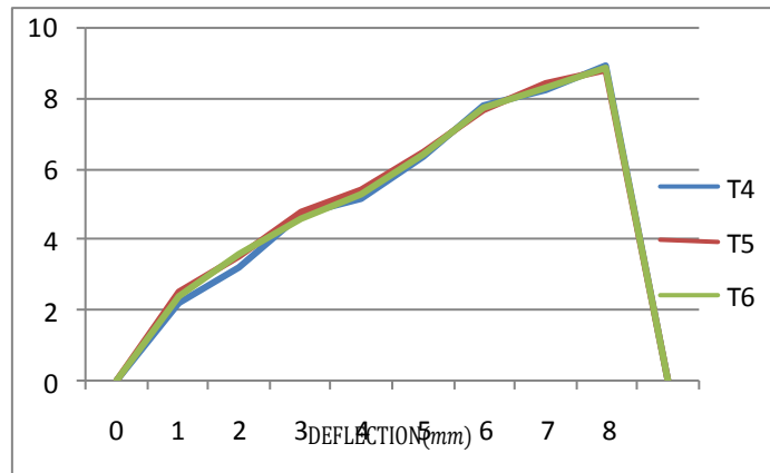
Fig 8. Load vs Deflection graph of Tensile test for composition 60%-40%
