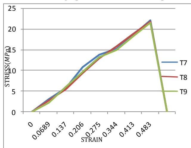
Fig 11. Stress vs Strain graph Tensile test for composition 55%-45%
