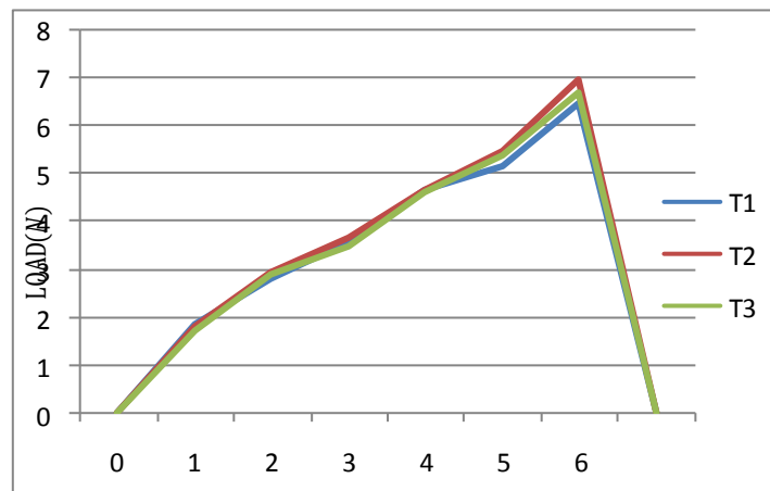
Figure 6: Load vs Deflection graph of Tensile test for composition 65%-35%
